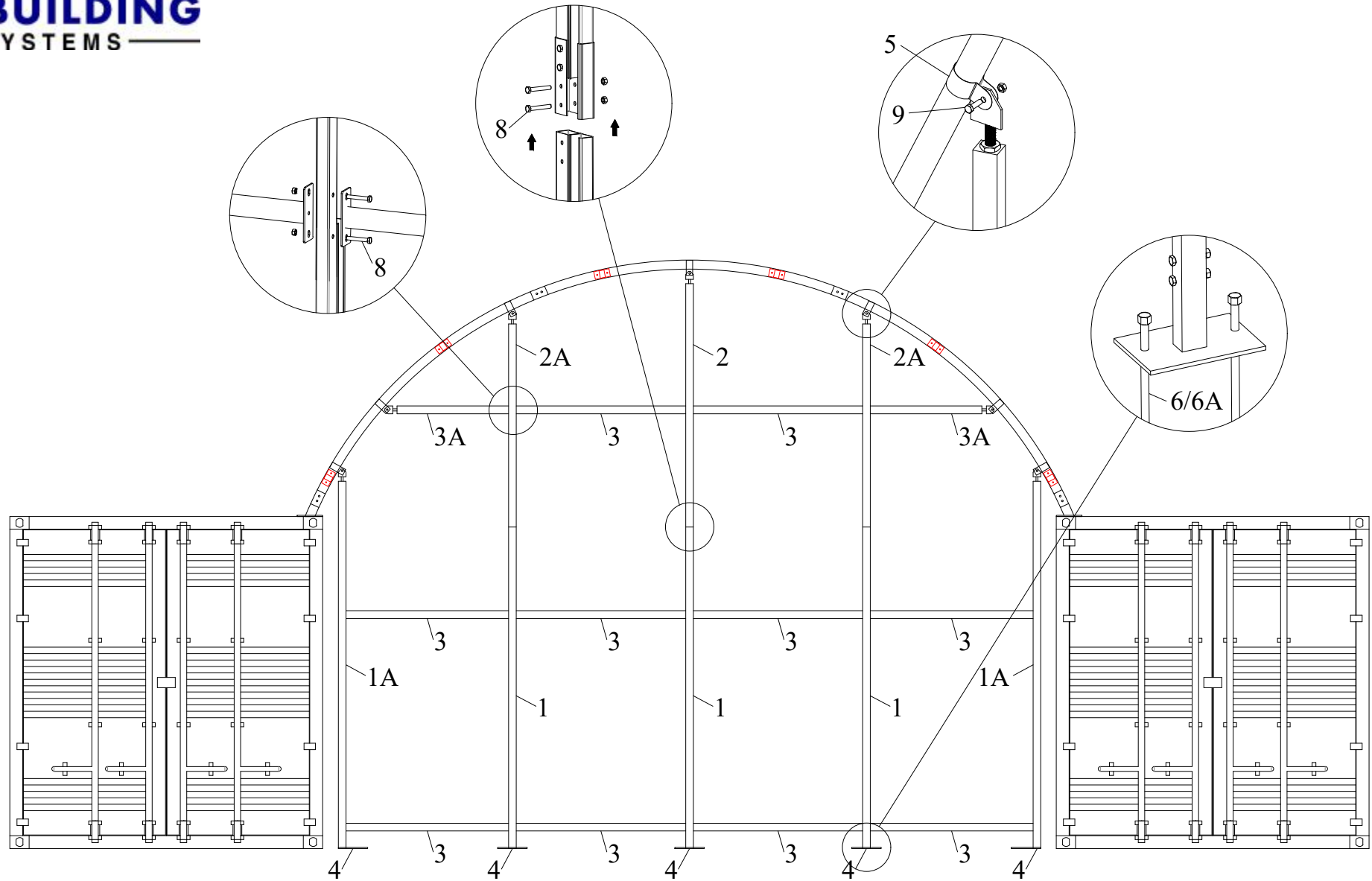
Figure.1 RAIL AND BEAM FOR BACK PANEL
